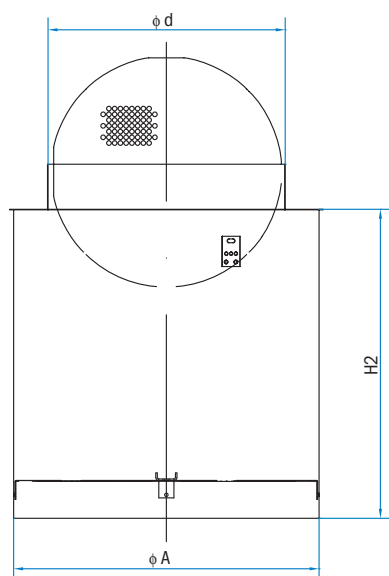
(V) top entry spigot
